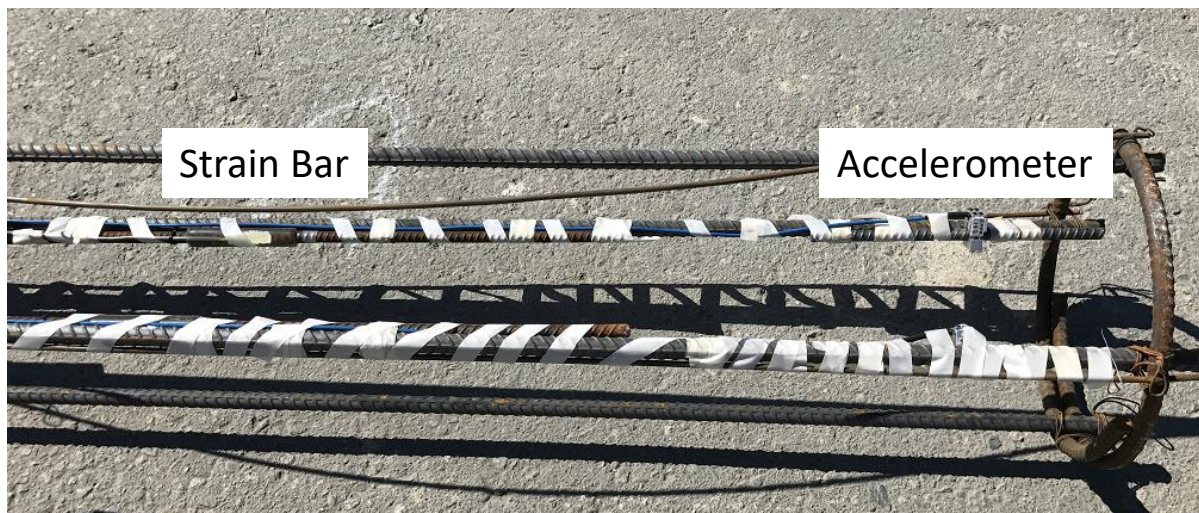
Figure 3 Sister bar strain sensor and accelerometer
