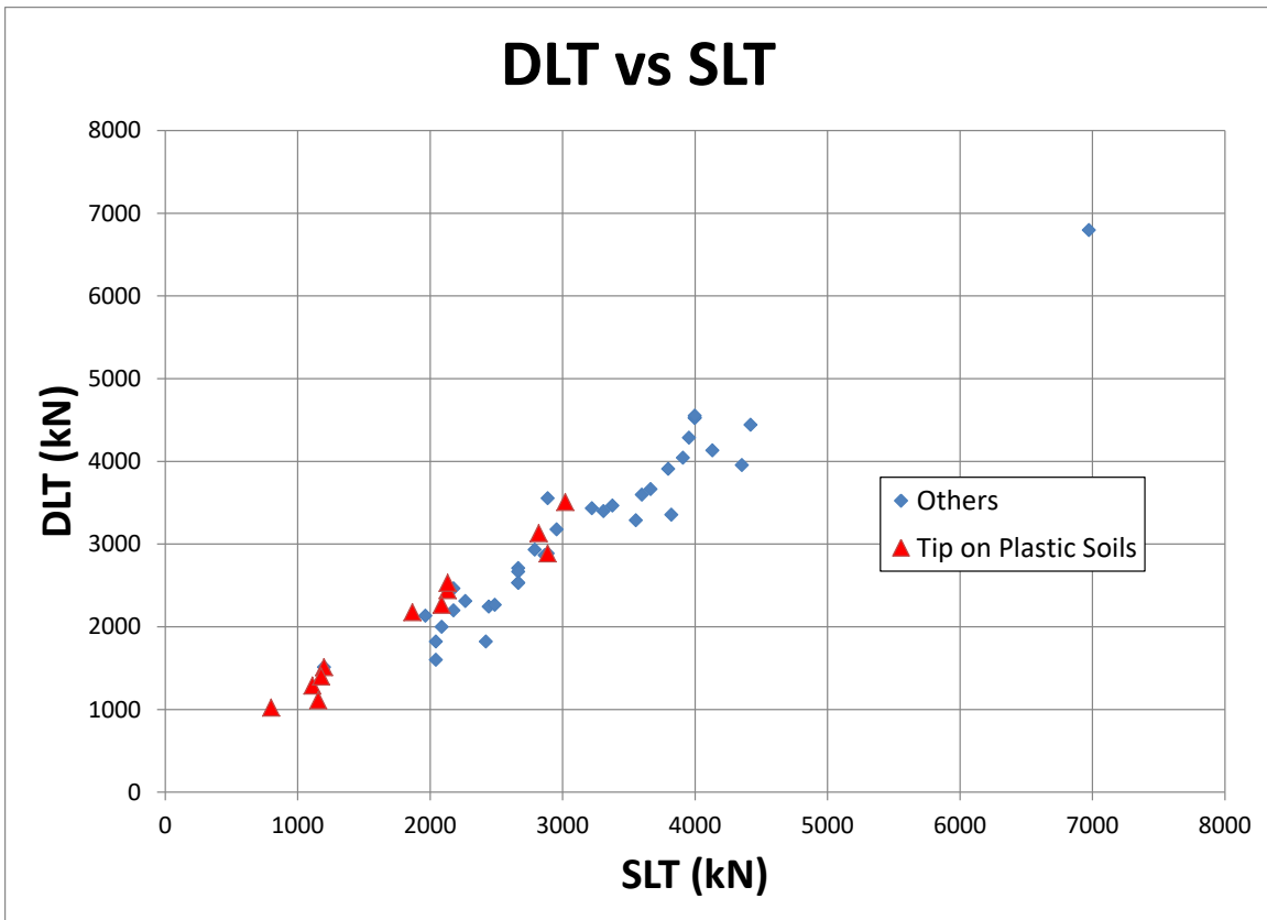
Figure 8 DLT vs SLT correlation separating piles tipped in high plastic soils.
