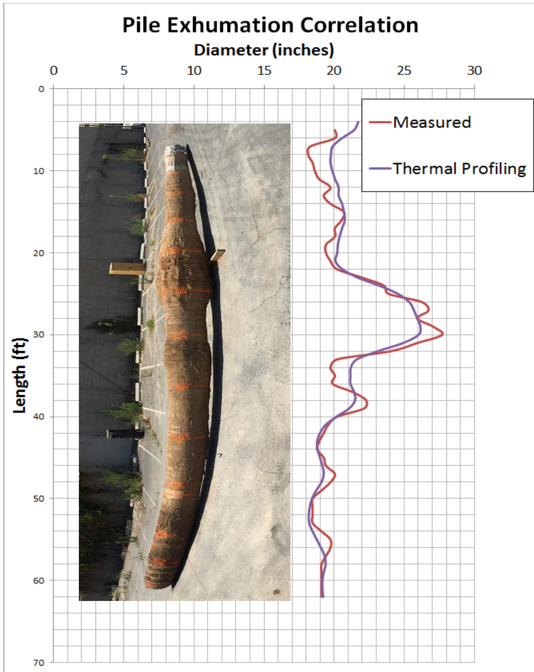
Figure 5 Thermal Profiling correlation of exhumed pile (1 ft = 0.3048 m)
