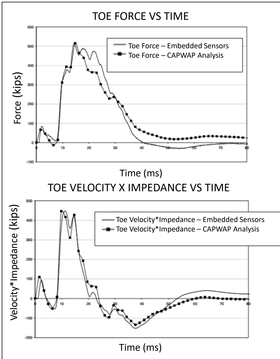
Figure 6 Signal matching on ACIP pile at toe [7] (kip=4.45 kN)
