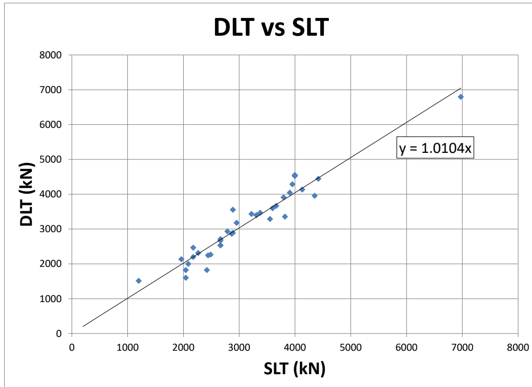
Figure 7 Dynamic versus static capacity for 47 ACIP test piles
