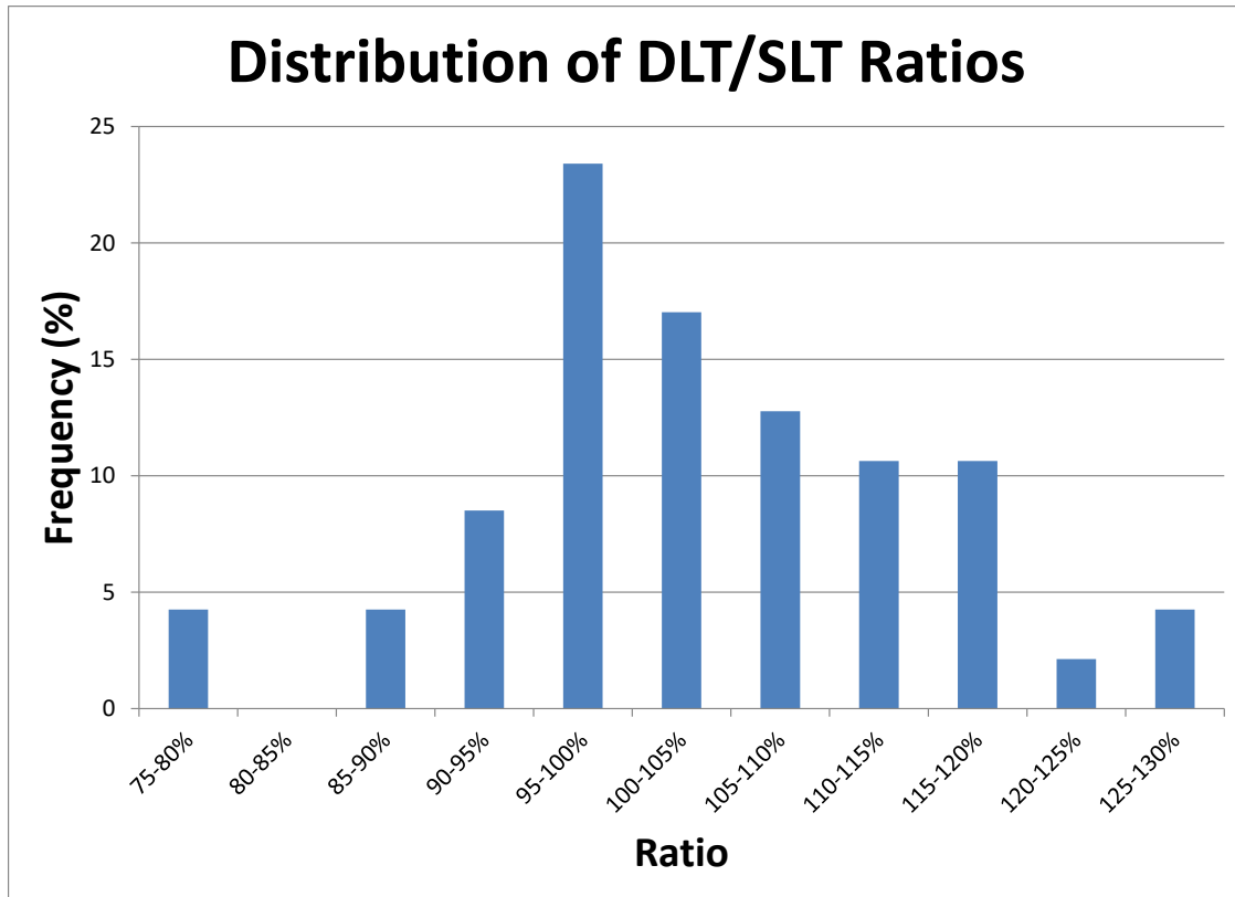
Figure 9 Distribution of ratios of DLT to SLT on ACIP Piles.
