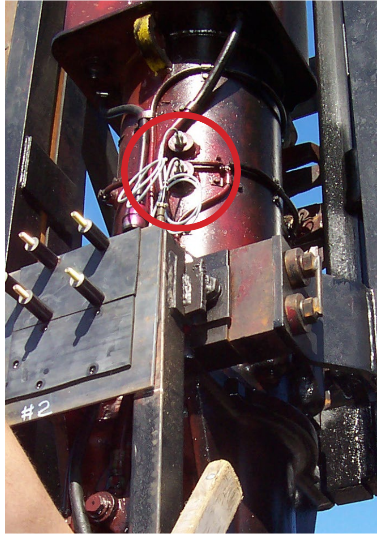
Proximity Switches
